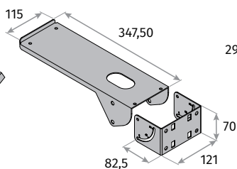
SOLAR PANEL FIXING SUPPORT
